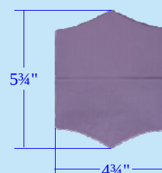
標準三尖袋蓋模效果及尺寸 Effect and Dimensions of Standard Triangular Bottomed Pocket Flap Mould
